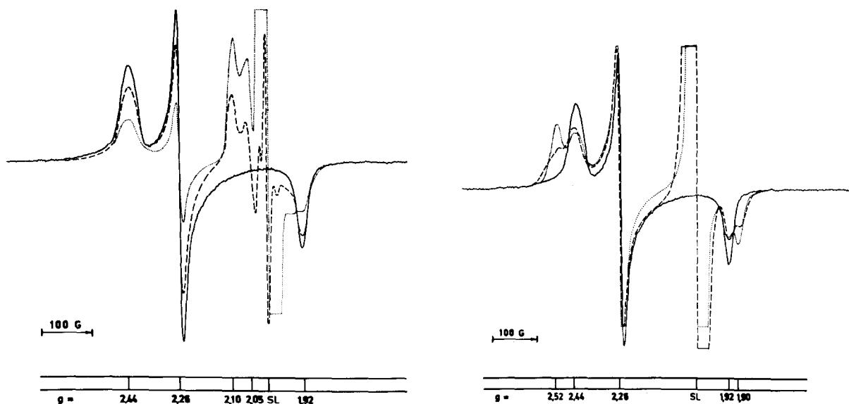
Fig. 3. EPR spectra of ferric low spin P -450 in presence of spin labelled n -alkylamines. (Microwave power, 20 mW; modulation, 12.5 G; T , -190^\circ\text{C} .) (A) — (—) without substrate; (---) m = 1 , [S_0] 2.5 \cdot 10^{-4} M; (·····) m = 1 , [S_0] 5 \cdot 10^{-3} M. (B) — (-----) m = 2 , [S_0] 5 \cdot 10^{-3} M; (·····) m = 10 , [S_0] 5 \cdot 10^{-3} M.
